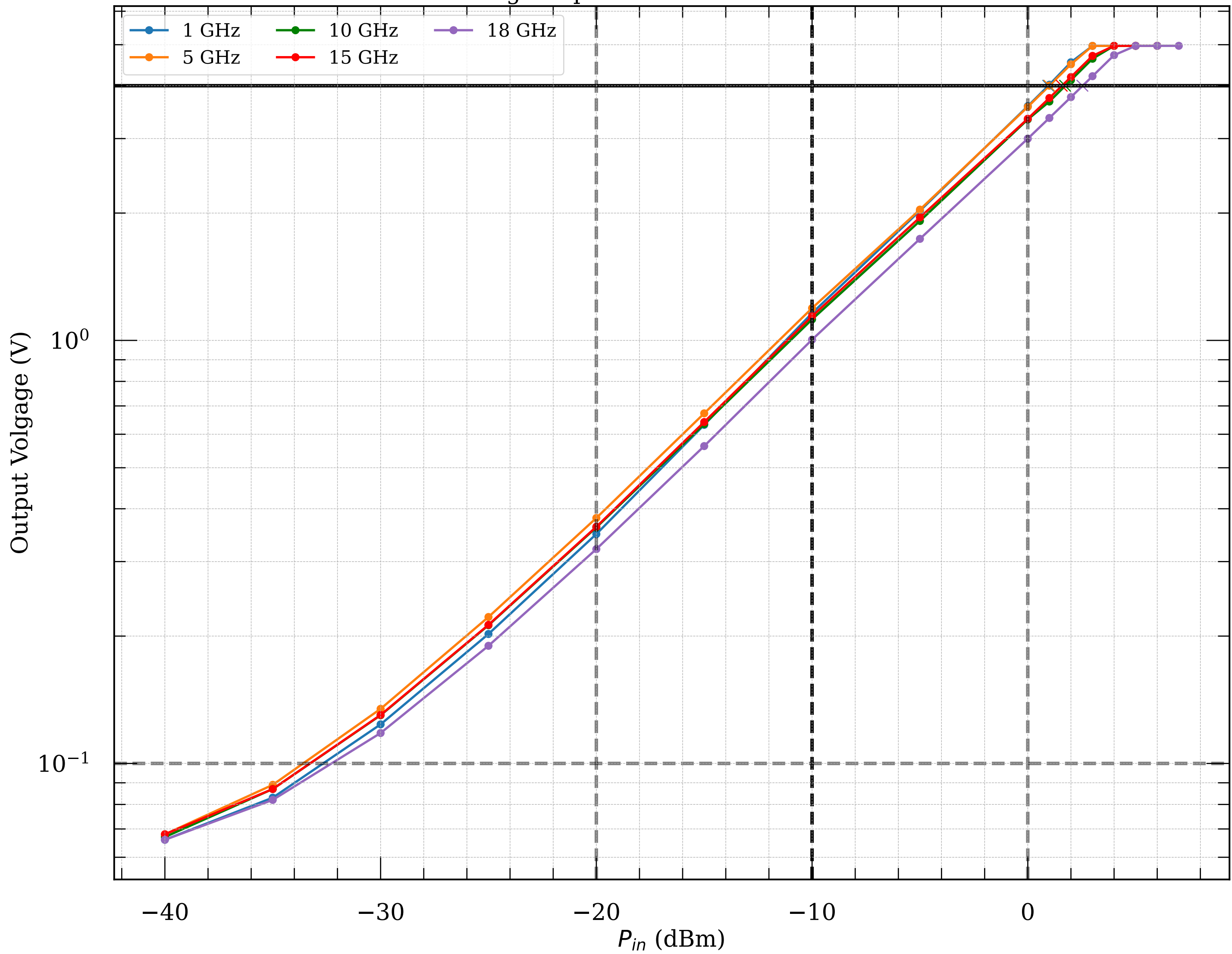
Measured voltage-to-power curve of detector module012v2
